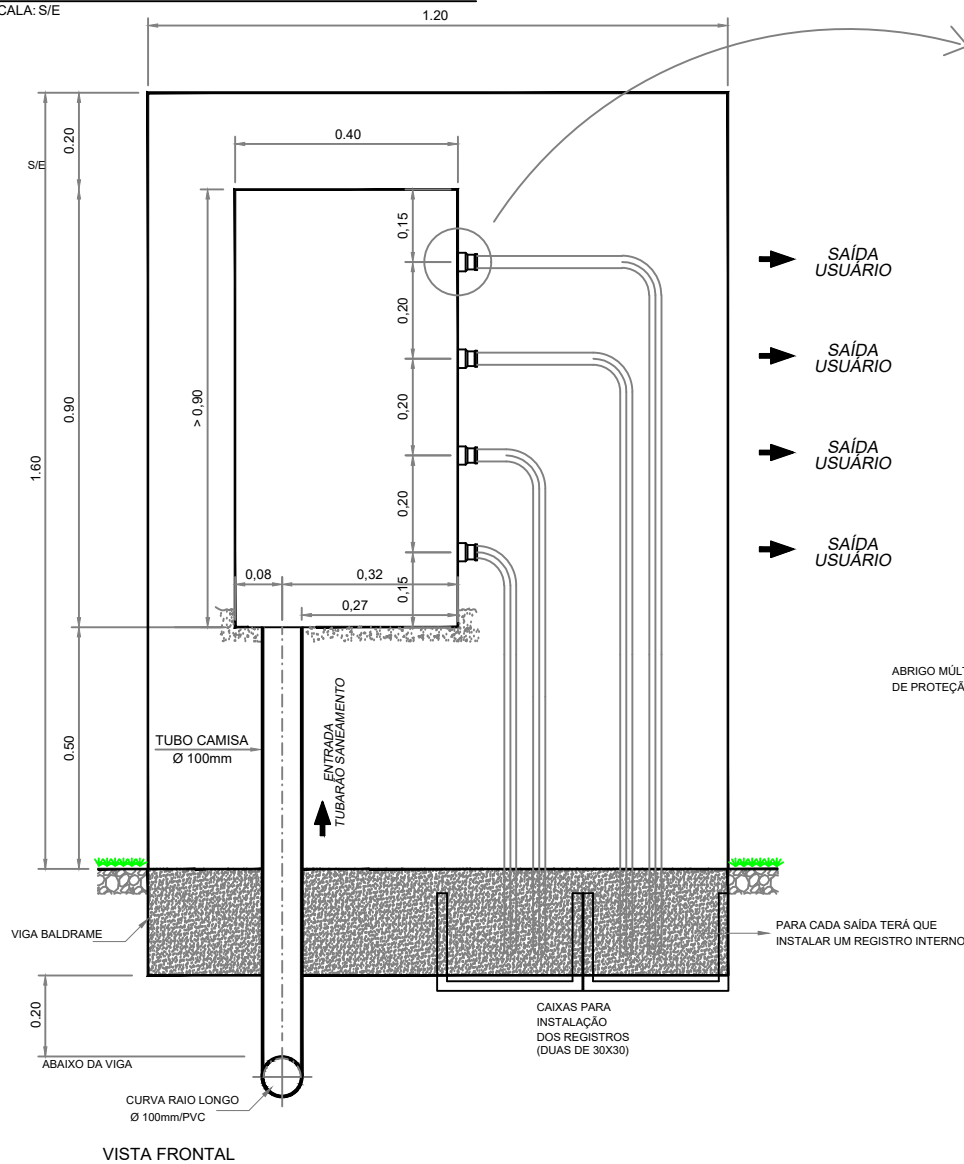
VISTA FRONTAL
